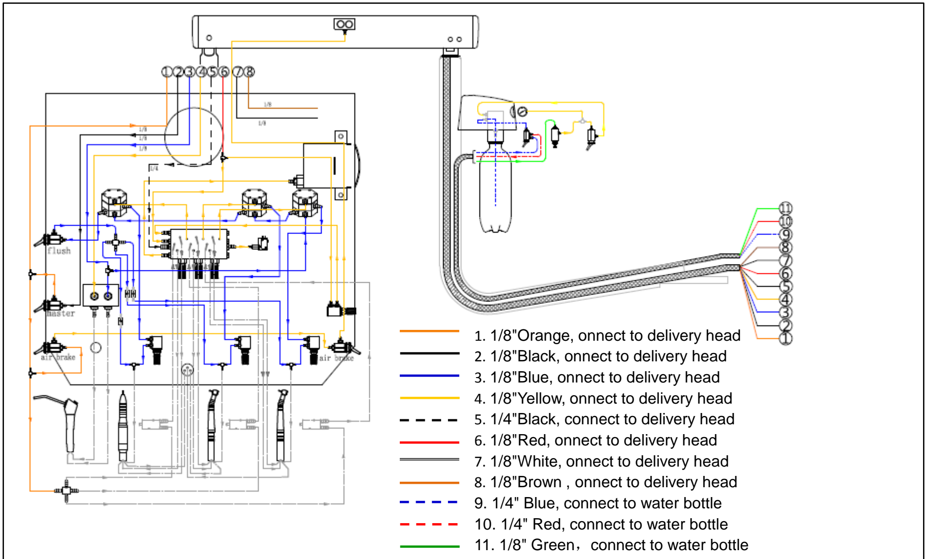
Figure 37 Water & Air diagram (delivery head)
